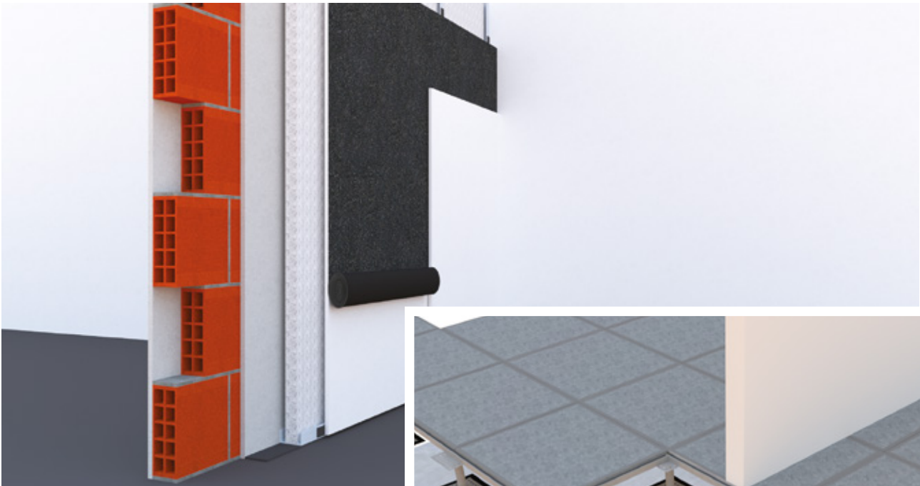
↑ Acoustic insulation with massive material insertion between two plasterboard panels. Isolmant Telogomma Classic can be applied at the head of the slab and easily cut at the base.
