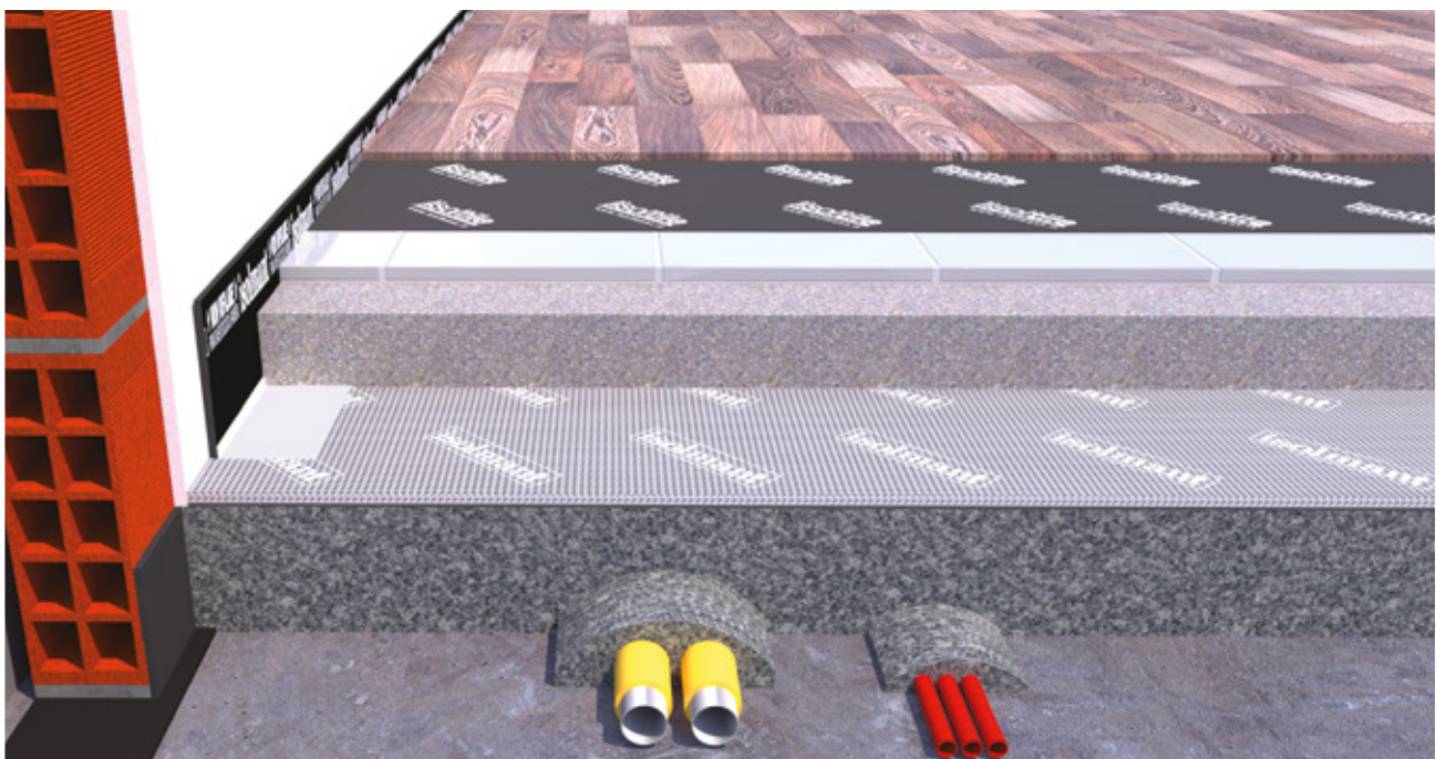
↑ With IsolTile AD, equipped with a positioning adhesive layer on the underside, it is possible to install in hybrid (or semi-floating) mode directly on existing flooring.
